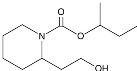
Figure 3: Picaridin
