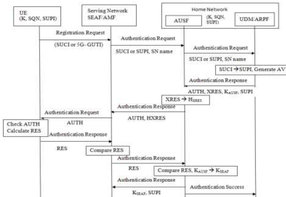
Figure 4: 3GPP 5G-AKA
