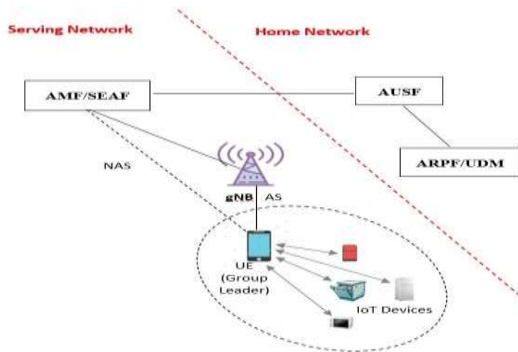
Figure 3: Security architecture of 5G-IoT
