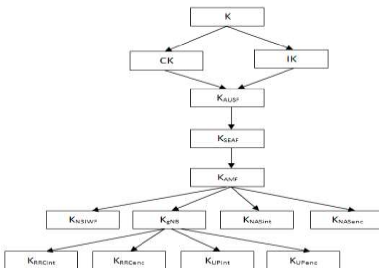
Figure 5: Keys generated during 3GPP 5G-AKA
