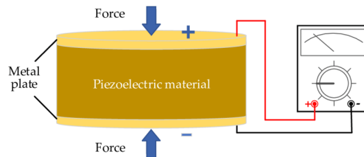
Fig: 3 Pizeo electric sensor
