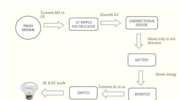
Fig:1 Block diagram of piezoelectricity
