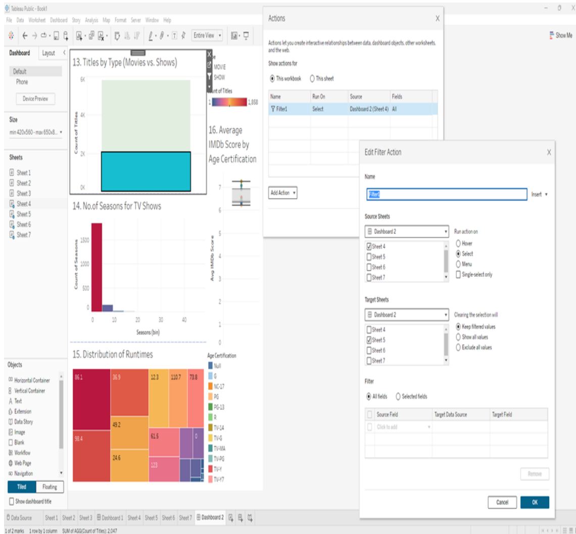
Fig.31: Filter Action
