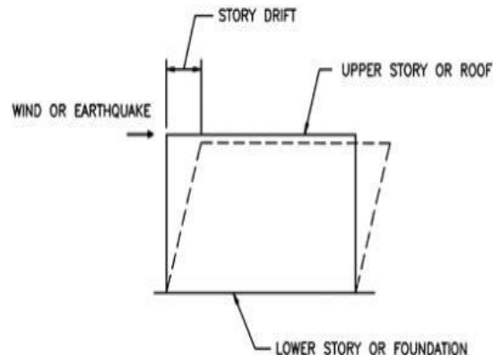
Figure 4.9 Story Drift
