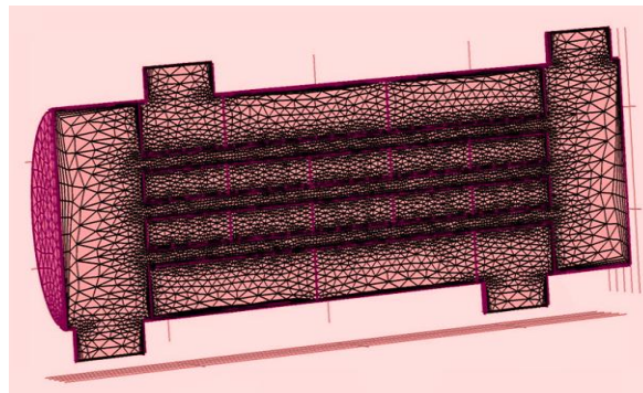
Fig. 2 Temperature plot of shell and tube heat exchanger
