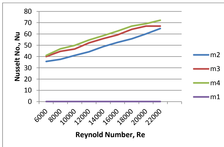
Fig 3 Plot of Nusselt number vs Reynolds Number
