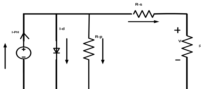
Fig 4: Equivalent circuit of photo-voltaic cell
