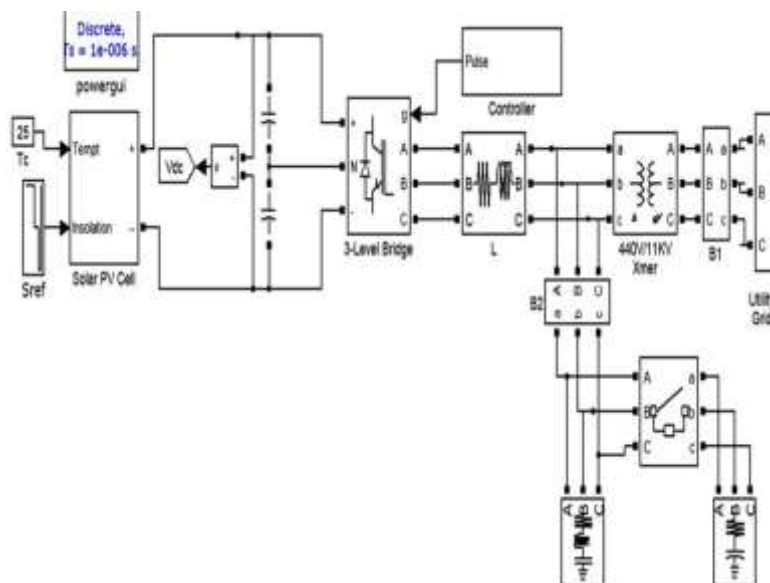
Fig 8: Simulink model of Grid connected Solar PV system
