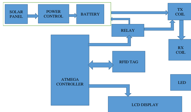
Figure 1: Block Diagram
