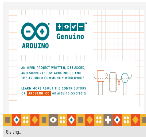
Figure 1: Arduino IDE
