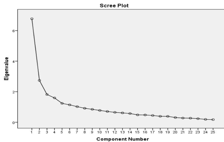
Figure 1. Scree Plot
