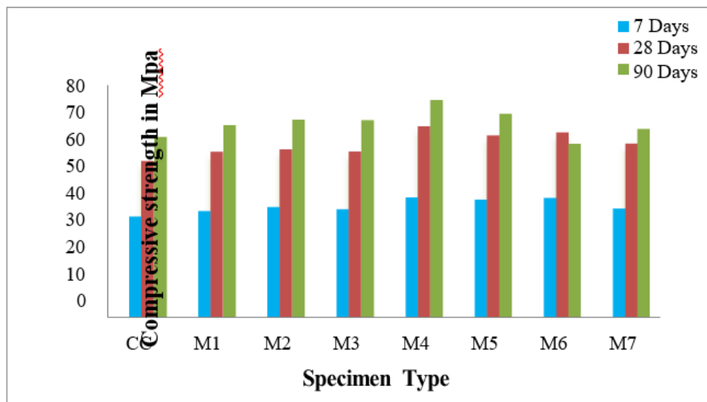
Figure 5.2 Compressive strength test result
