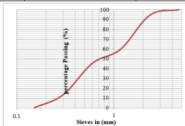
Figure 1 Grading curve of fine aggregate
