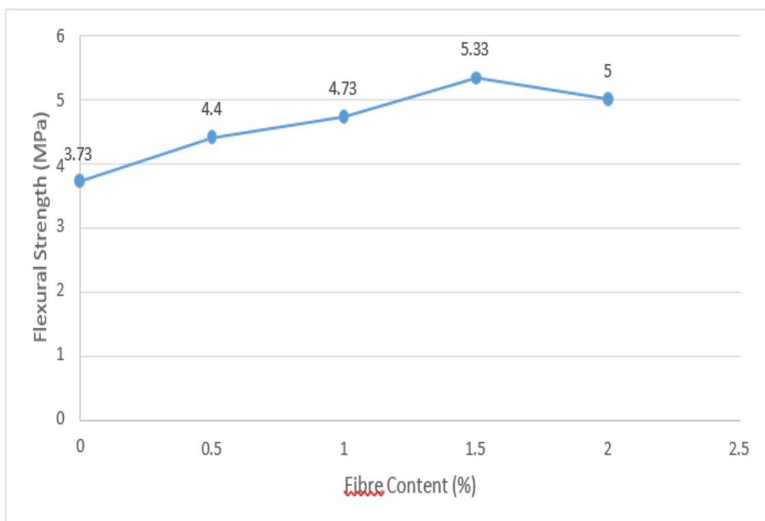
Figure 5.3: relationship between bending strength and concentration of fibre after 7 days
