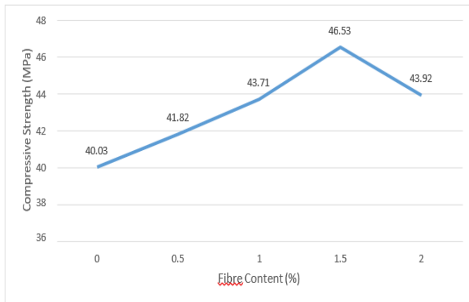
Figure 5.5: Examining the connection among compressive strength and fibre content at the 28-day mark.
