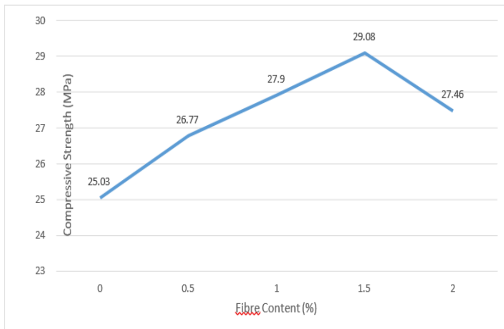
Figure 5.1: relationship between strength in compression and concentration of fibre after 7 days
