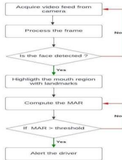
Fig 5. Process of Yawn Detection
