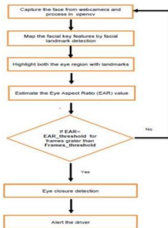
Fig 2: Process Flow of Eye Closure Detection
