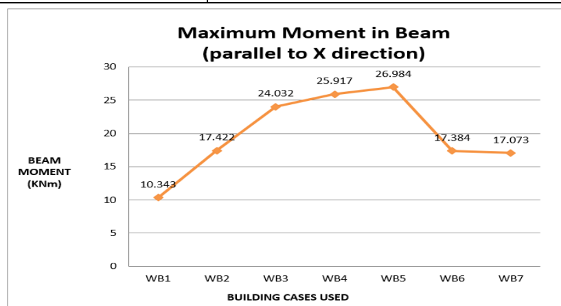
Fig. 6: Maximum Bending Moment in beams parallel to X direction for all wall belt cases
