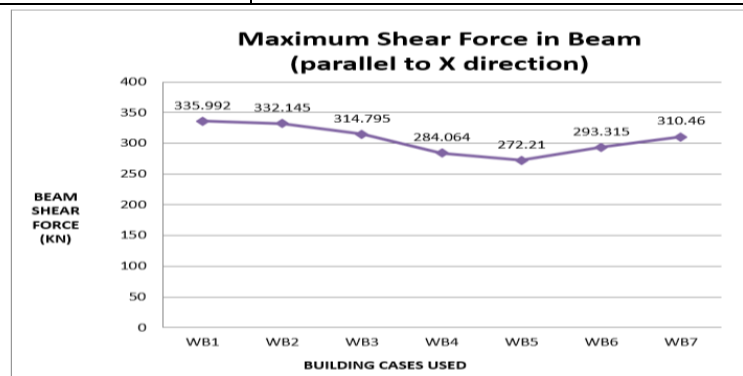
Fig. 4: Maximum Shear Forces in beams parallel to X direction for all wall belt cases
