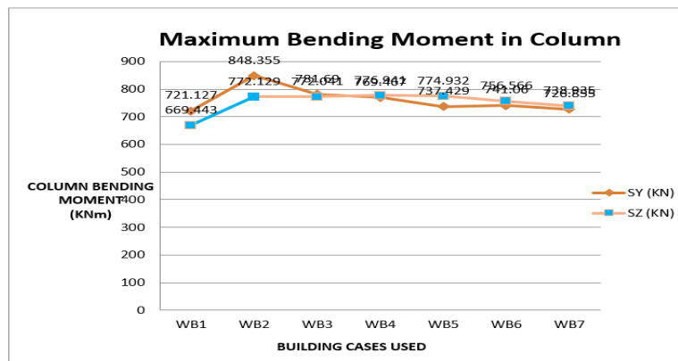
Fig. 3: Maximum Bending Moment in Columns for all wall belt cases
