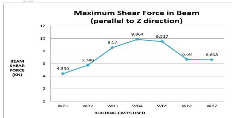
Fig. 5: Maximum Shear Forces in beams parallel to Z direction for all wall belt cases
