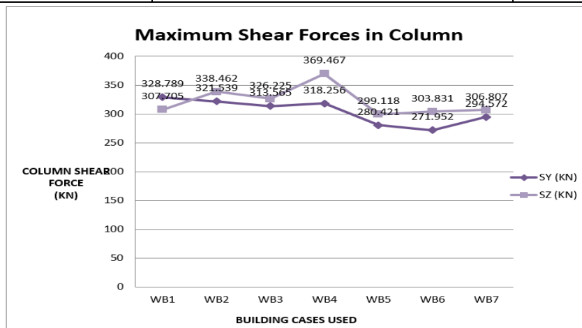
Fig. 2: Maximum Shear Forces in Columns for all wall belt cases
