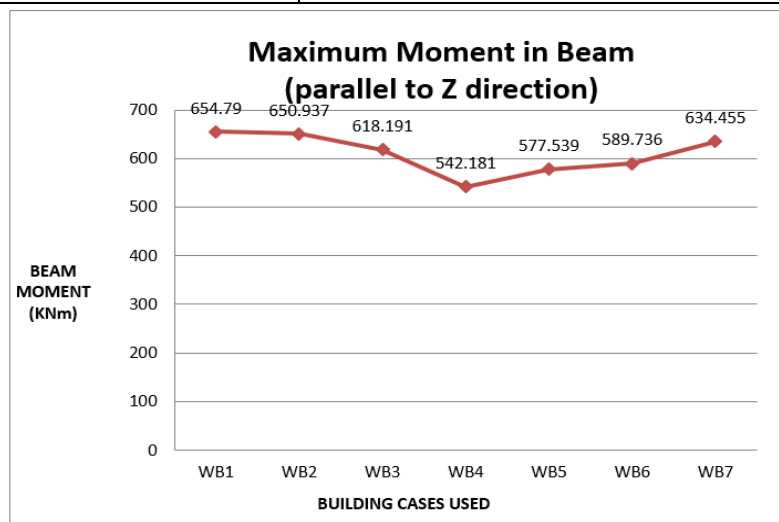
Fig. 7: Maximum Bending Moment in beams parallel to Z direction for all wall belt cases
