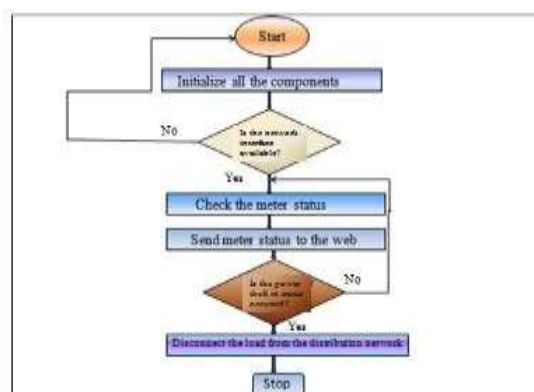
Figure 2. Process Flow
