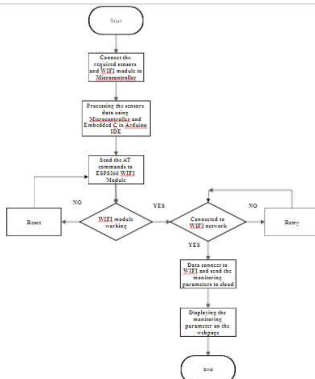
Figure 3. Software flow of meter reading
