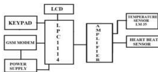
Fig.1 Block Diagram of Health Monitoring System
