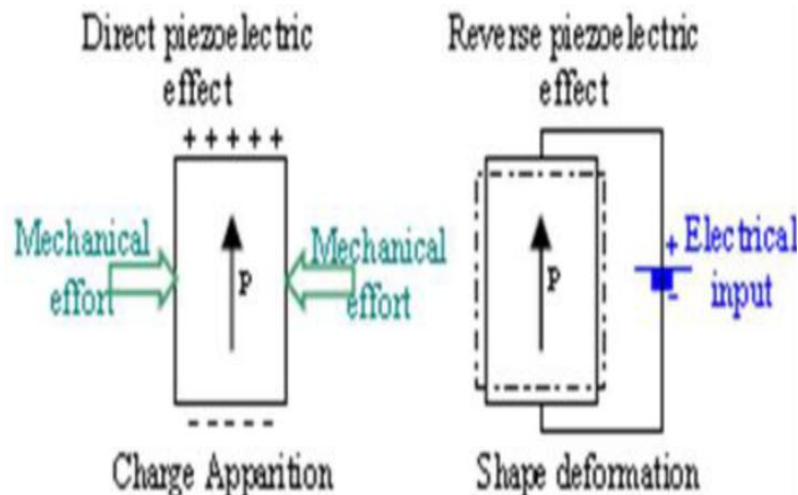
Fig1.1: Electromechanical conversion via piezoelectricity phenomenon
