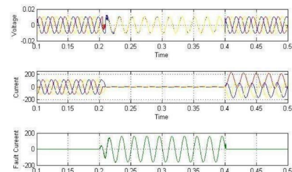
Figure9: Temporary Line-Line-Line-Ground Fault
