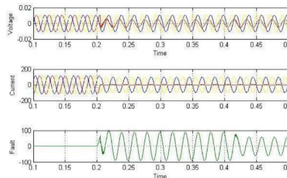
Figure8: Permanent Line to Ground Fault
