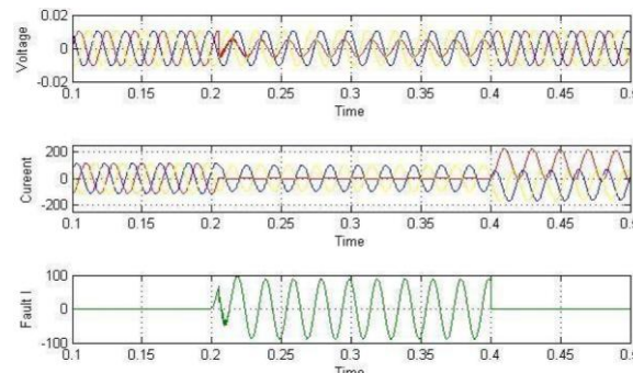
Figure7: Temporary Line to Ground Fault
