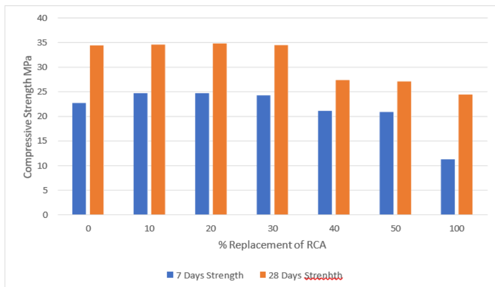
Fig 5.4 Average Strength Variation for Various % Replacement of RCA in Cube
