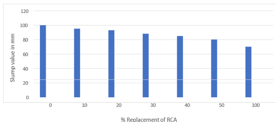
Fig 5.1 Slump Value of Different % Replacement of RCA
