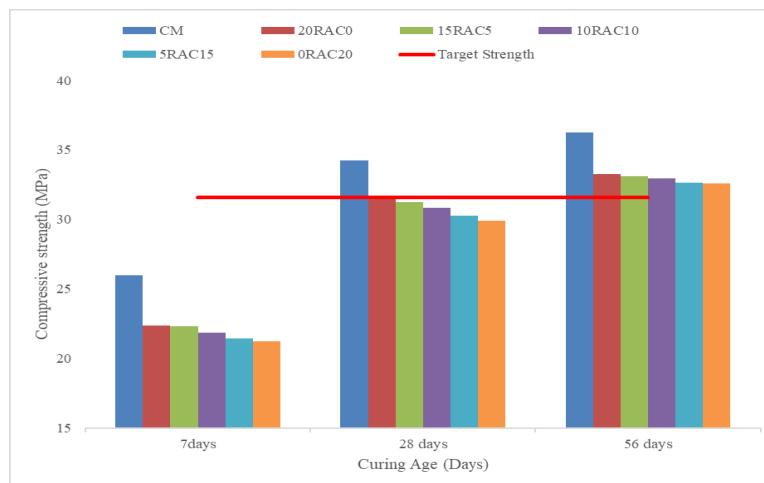
Fig. 5.5 Variation of Compressive strength
