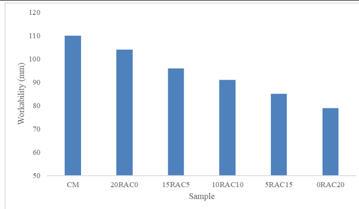
Fig. 5.4 Graph illustrating the workability of several samples.
