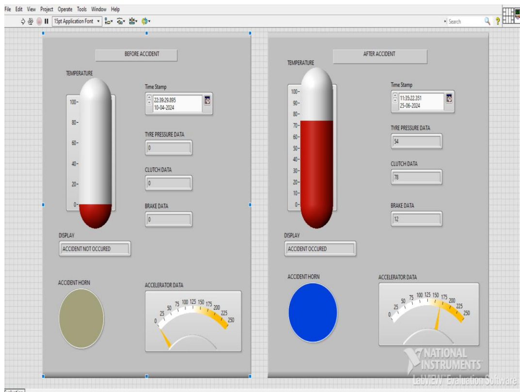
Fig. 2. Output of the system (LABVIEW)
