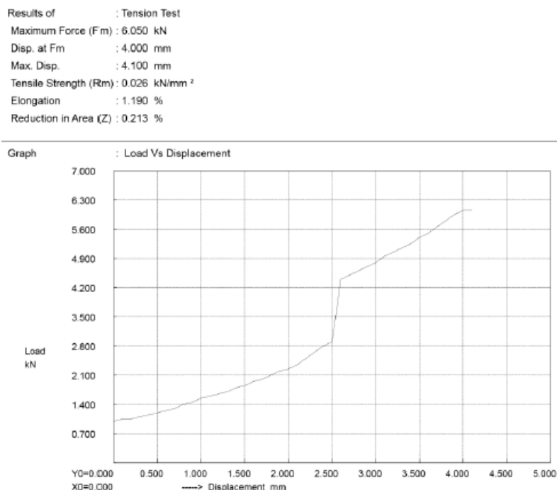
Figure 1: Test Results for Tensile Test
