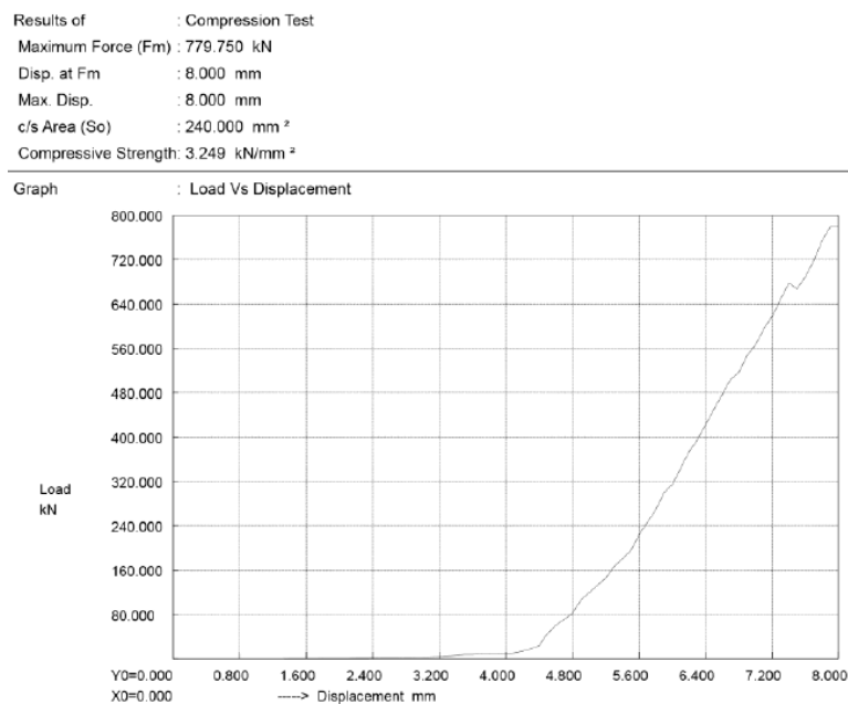
Figure 3: Compression Test Results
