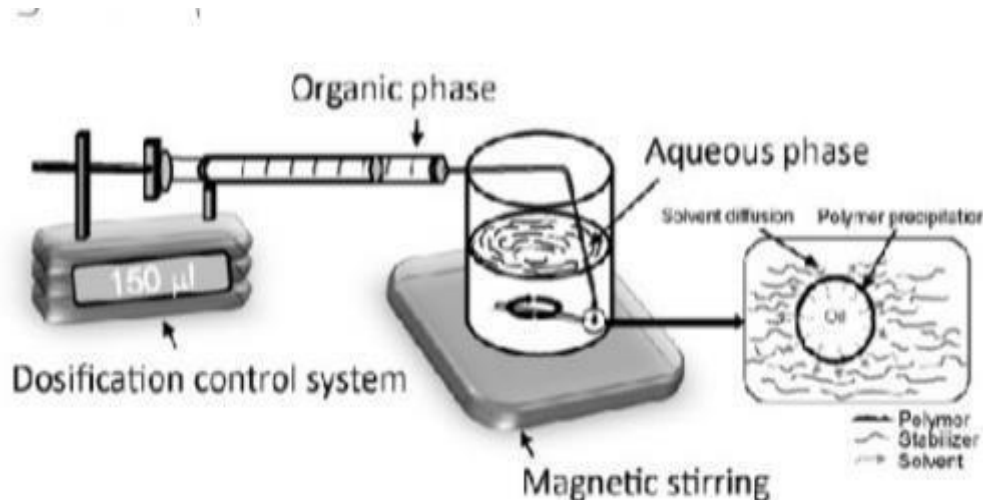
Preparation of nanocapsule by precipitation method
