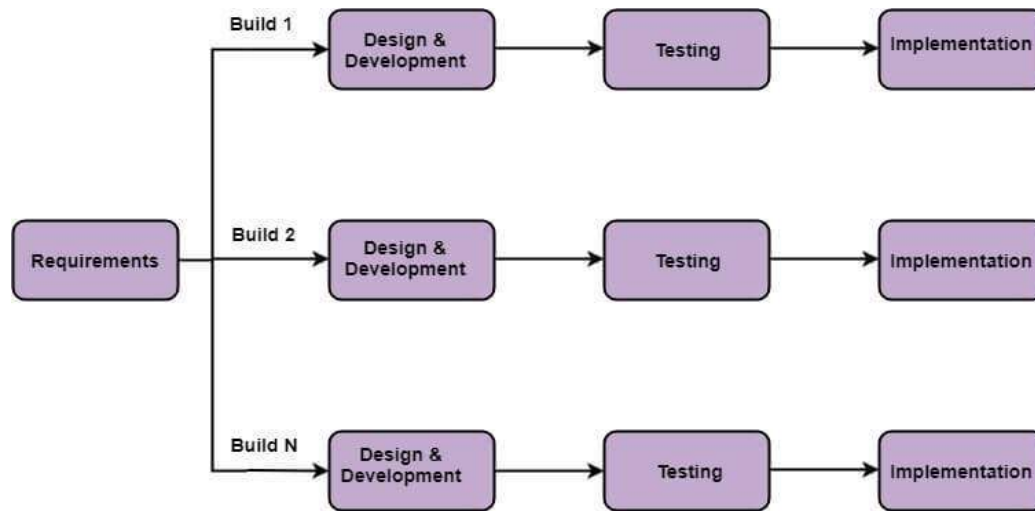
Fig 2.2 Incremental model
