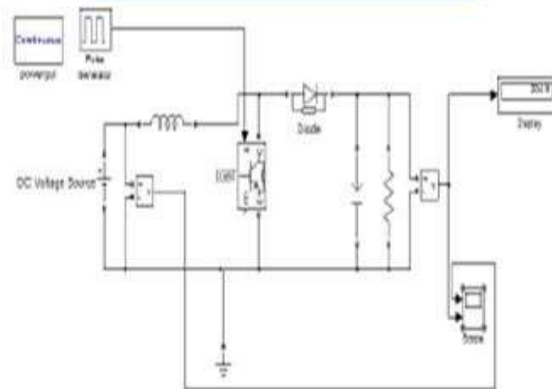
Figure 2: Matlab – Simulink circuit for Boost Converter
