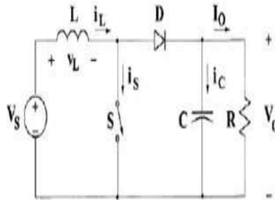
Figure1: Step-up or Boost Converter
