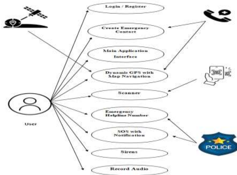
Figure 1: Use Case Diagram of Women Safety App
