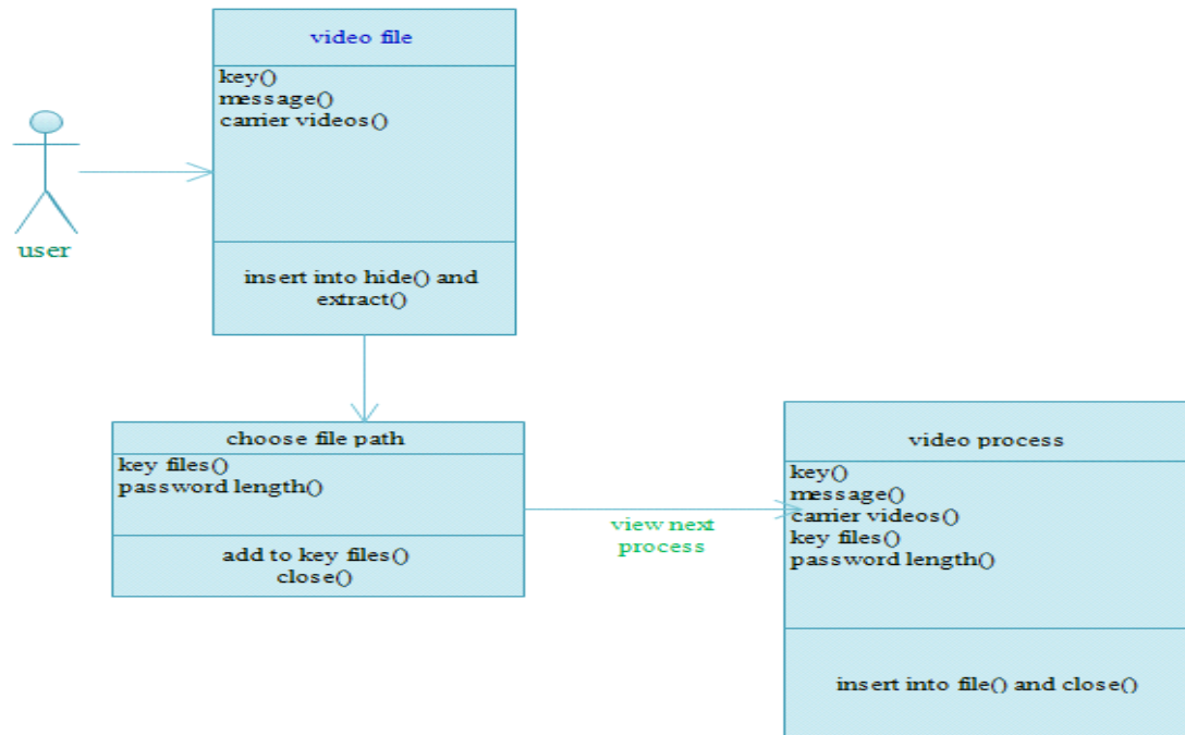
Figure 3. Class Diagram
