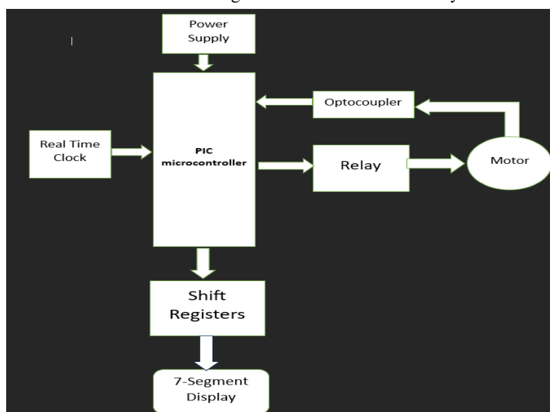
Figure 1. smart timer system for industrial automation system
