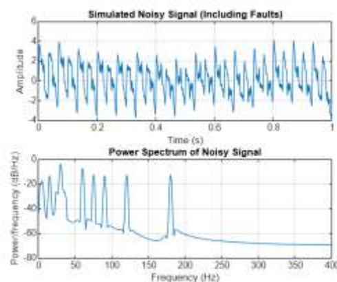
Figure 2: Simulated Noise signal followed by its Welch Transform
