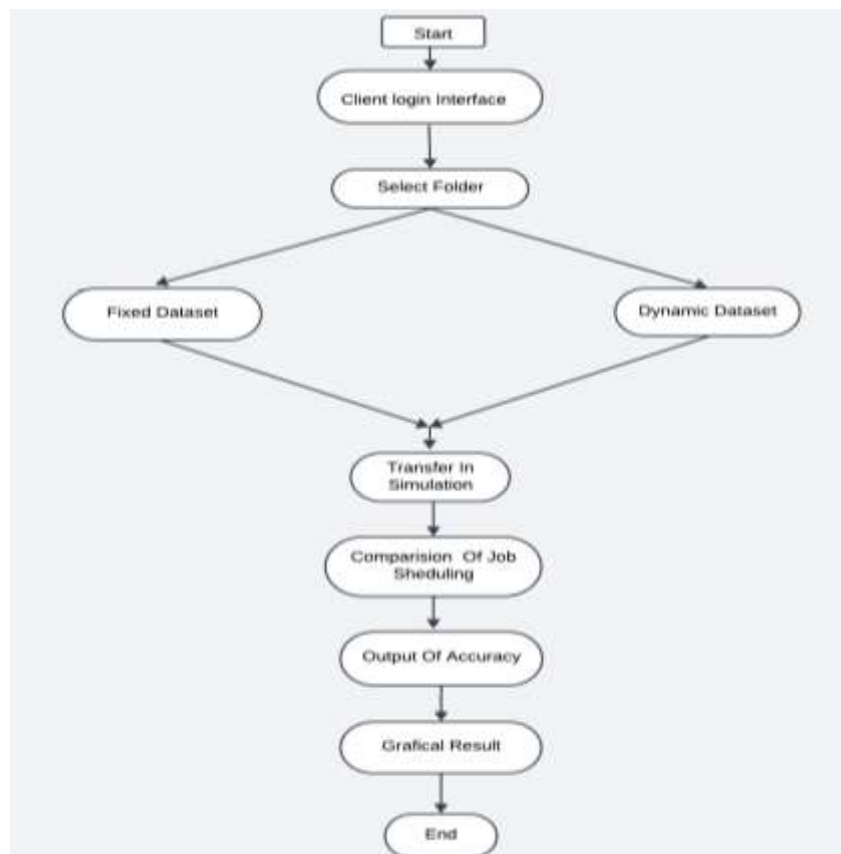
Fig 4.1: System Architecture
