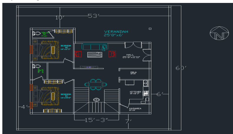
Fig 1. Ground floor plan of villa
