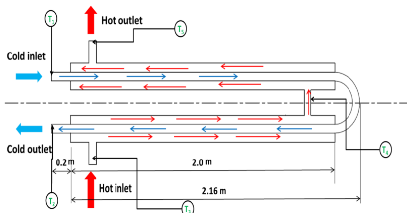
Figure: -1 Schematic representation of double pipe U-bend heat exchanger
