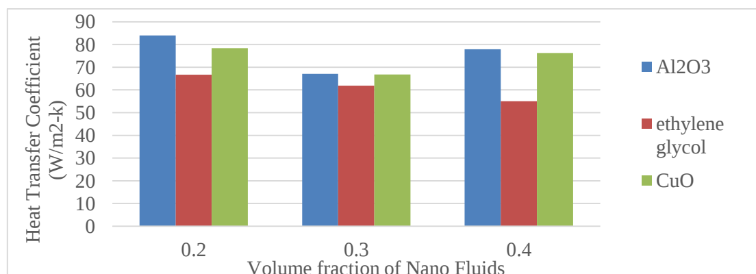
Figure: 5 Heat Transfer Coefficient vs. Nano fluids
