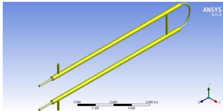
Figure:-2 Geometry modelling of 2-Pass Double Pipe in ANSYS work bench
