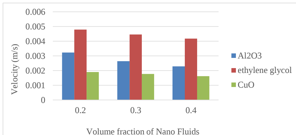
Figure:-4 Velocity vs. Nano fluids
