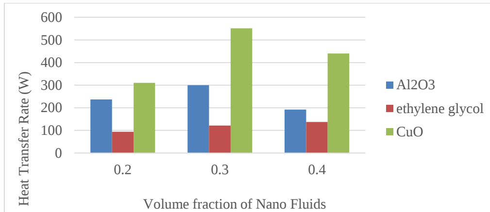
Figure:-6Heat Transfer Rate vs. Nano fluids
