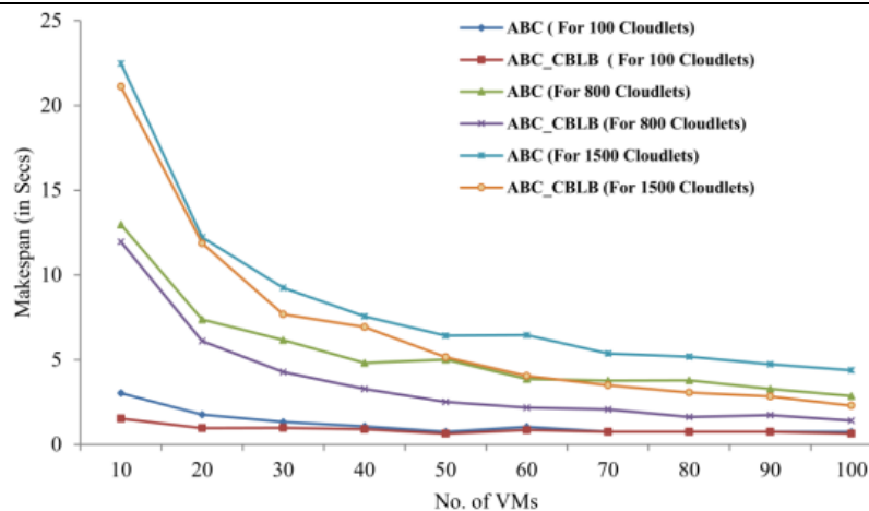
Figure 2: Different Numbers of VMs
