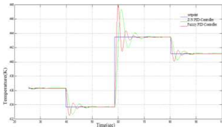
Fig. 8. Servo Response Comparison of Ziegler-Nichols PID-Controller and Fuzzy PID-Controller
