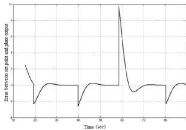
Fig. 10. Error Response for APSO PID-Controller
