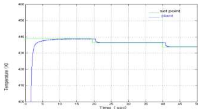
Fig. 7. Servo Response of Trial and Error Method
