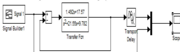
Fig. 3. Simulink Block Diagram for Closed loop systems
