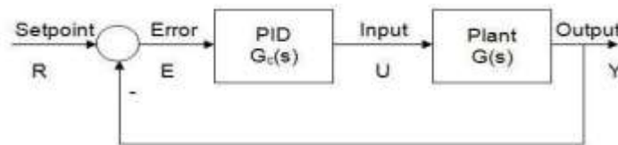
Fig. 2. Block diagram of PID controller with G(S) Plant
