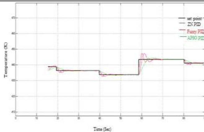
Fig. 9. Servo Response for APSO PID-Controller
