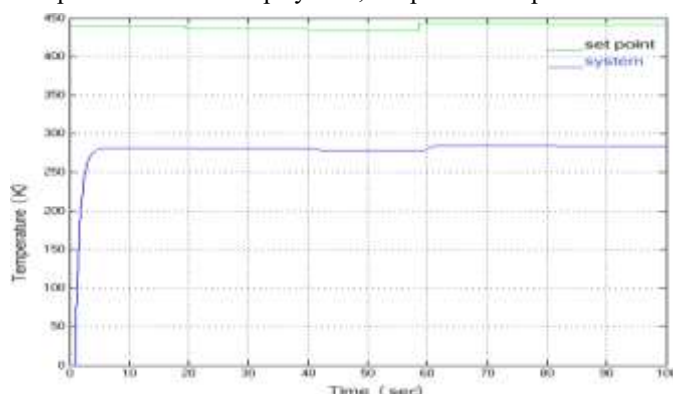
Fig. 6. Servo Response of Closed loop Systems
