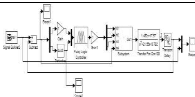
Figure 5 , shows the Simulink block diagram of fuzzy PID- Controller
