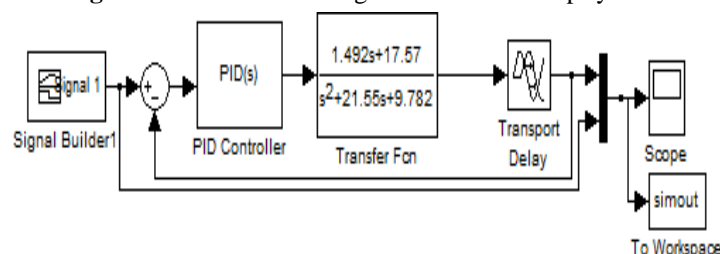
Fig. 4. Simulink Block Diagram for PID-Controller
