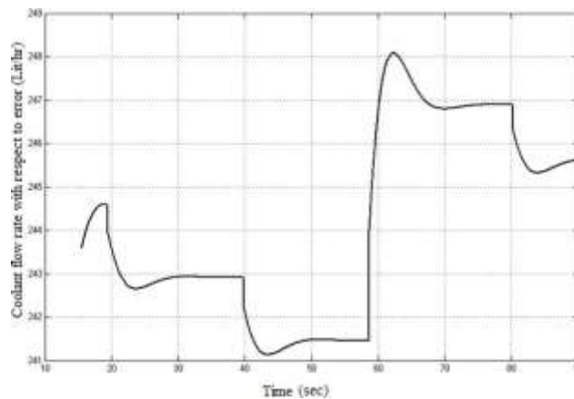
Fig. 11. Coolant Flow Rate with respect to Error for APSO PID-Controller
