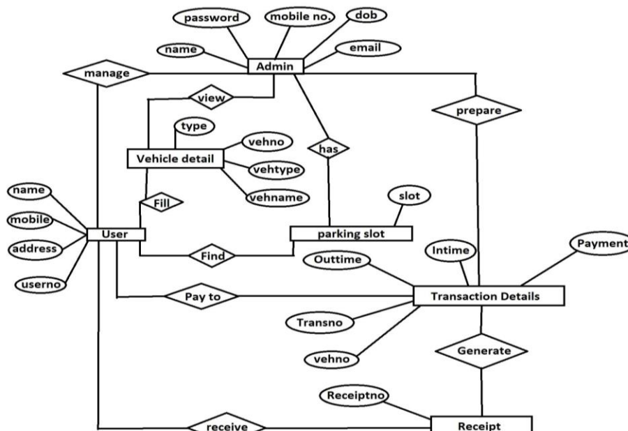
Figure 1: E-R Diagram
