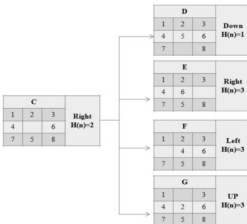
Figure 3: Traversing at Depth 3.
