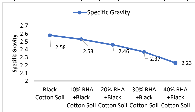
Fig. 8. Specific gravity of Soil with altered RHA percentages.
