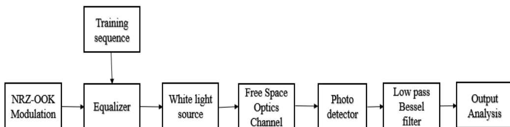
Fig 1 : Block diagram for the pre equalized VLC system
