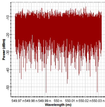
Fig 9 : White light spectrum for center frequency 550nm in Optical Spectrum Analyzer
